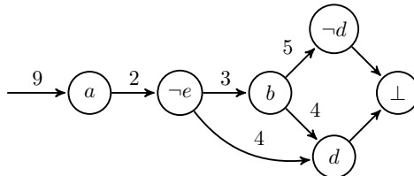
Figure 4.9: Conflict graph for step 14.
